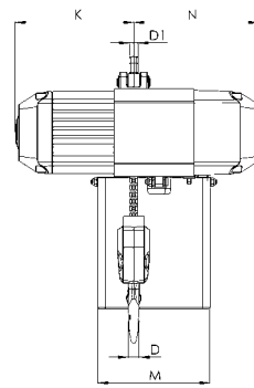
Model CPV/CPVF askı halkalı, 500 -2000 kg, çift zincir donamlı
