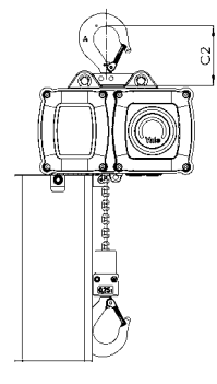
Model CPV/CPVF askı kancalı, 250 - 2000 kg
