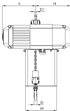
Model CPV/CPVF askı halkalı, 250 -1000 kg, tek zincir donamlı
