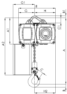
Model CPV/CPVF askı halkalı, 250 -1000 kg, tek zincir donamlı
